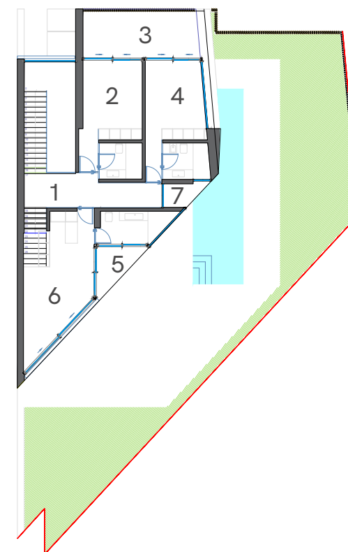
PISO 1 / FIRST FLOOR
